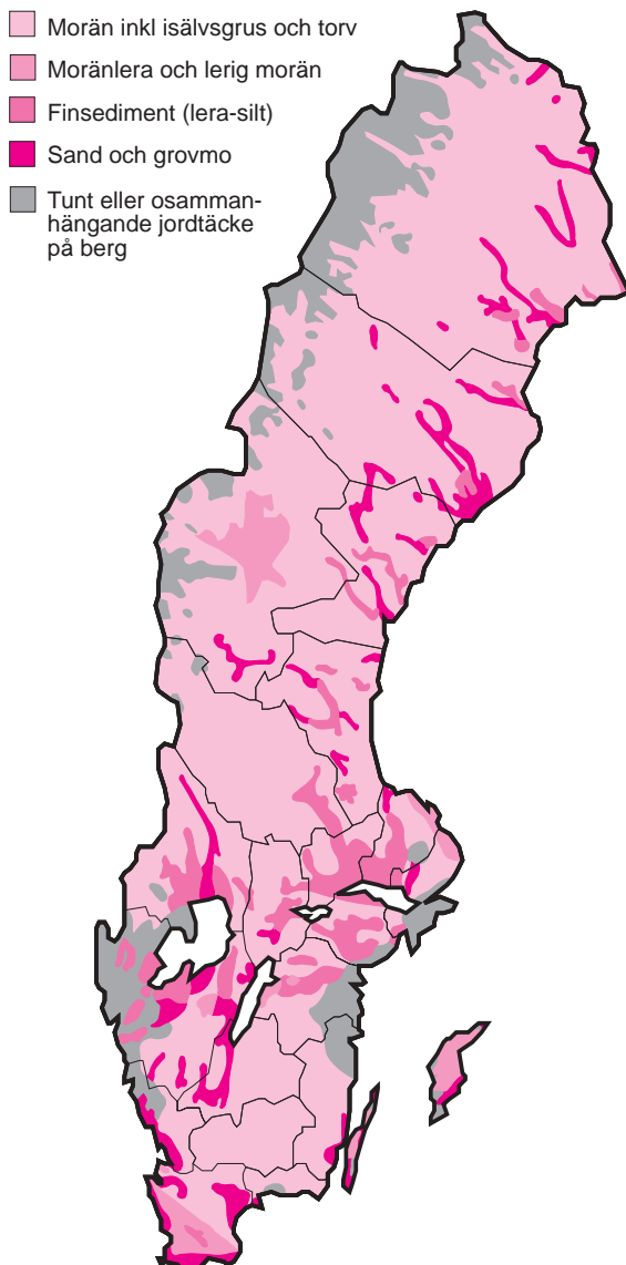
Figur 9 Jordarter
