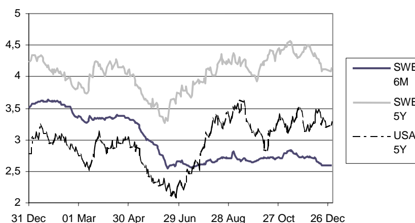
Swedish six-month/five year interest rates and US five-year interest rates during 2003, per cent
